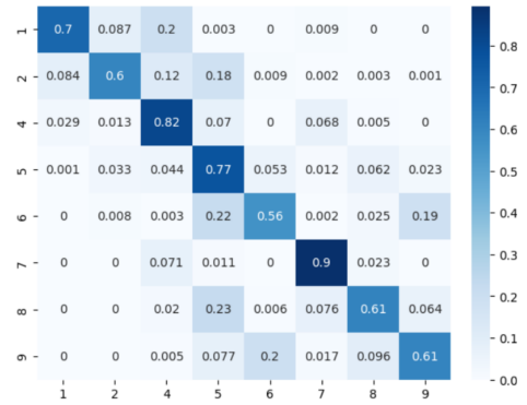
Fig. 3: Confusion matrix of the original (rows) and reconstructed (columns) H - \alpha classes.
