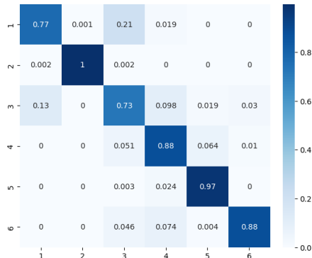
Fig. 5: Confusion matrix of the ground truth (rows) and predicted (columns) classes over the labeled classes.
