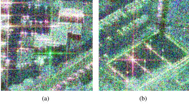
Fig. 2. Toulouse, RAMSES PolSAR data, X-band ( 150 \times 150 pixels). Colored composition in the Pauli basis of the target vector [k]_1-[k]_3-[k]_2 . Images containing a dihedral (a) and a narrow diplane (b).
