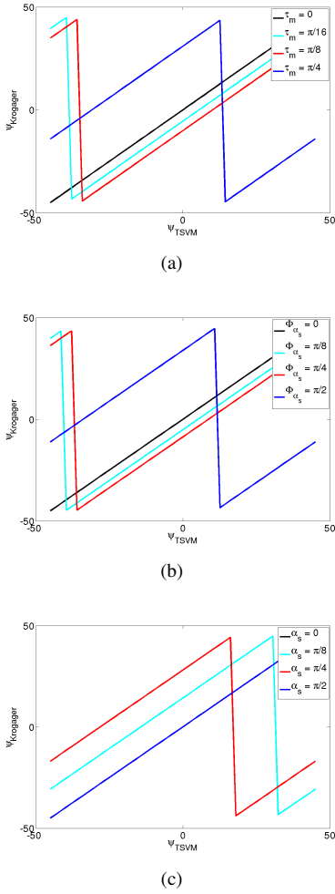
Fig. 1. Comparison between \psi_{TSVM} and \psi_{Krogager} : (a) as a function of \tau_m for \alpha_s = \pi/3 and \Phi_{\alpha_s} = \pi/3 , (b) as a function of \Phi_{\alpha_s} for \alpha_s = \pi/3 and \tau_m = \pi/8 and (c) as a function of \alpha_s for \Phi_{\alpha_s} = \pi/3 and \tau_m = \pi/8
